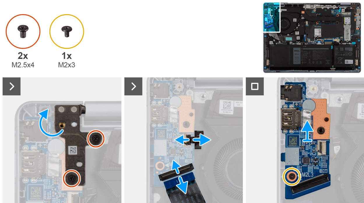
Figure 33. Removing the I/O board
