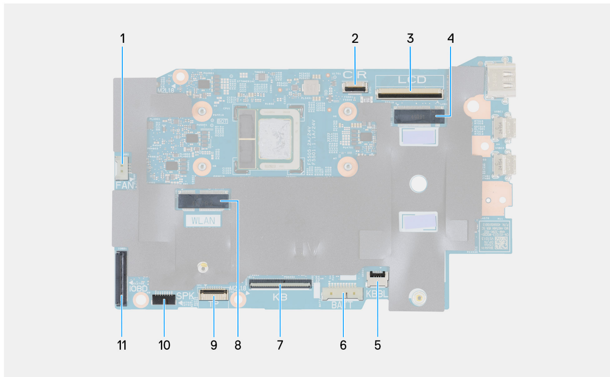
Figure 44. System board callouts
