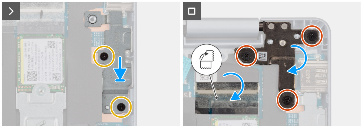
Figure 47. Installing the system board
