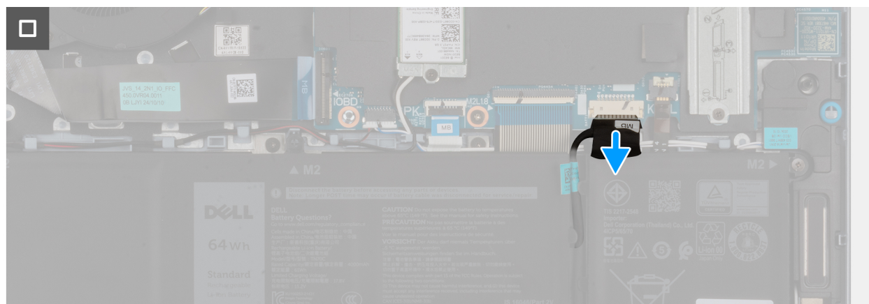
Figure 12. Disconnecting the battery cable
