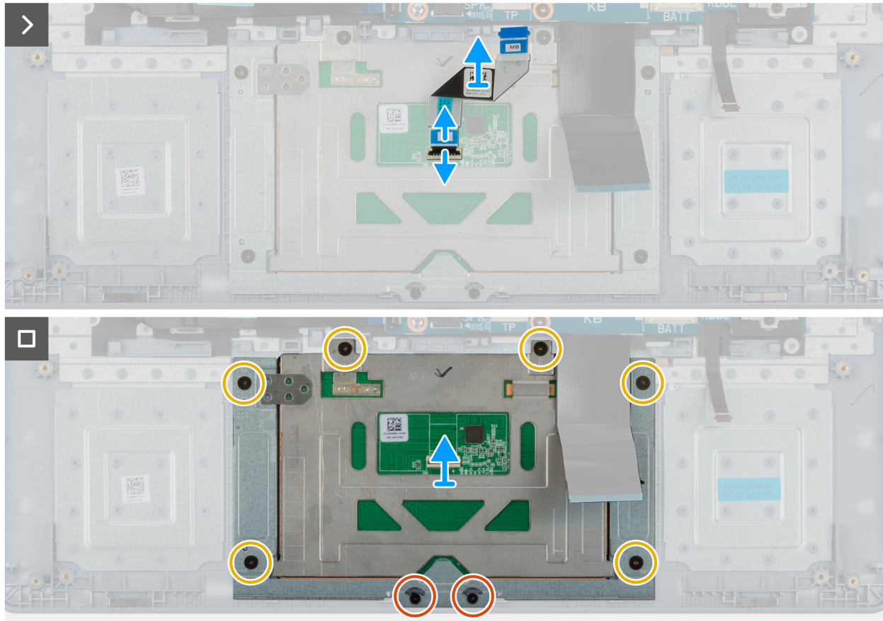
Figure 53. Removing the touchpad
