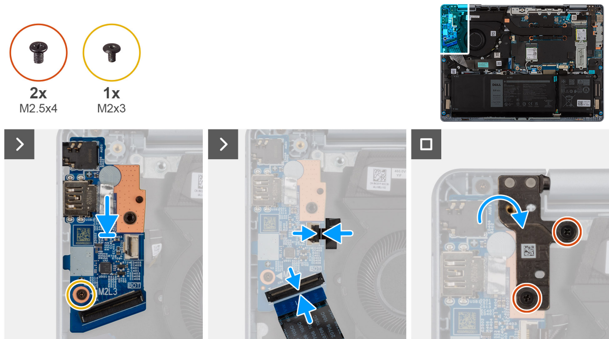
Figure 34. Installing the I/O board
