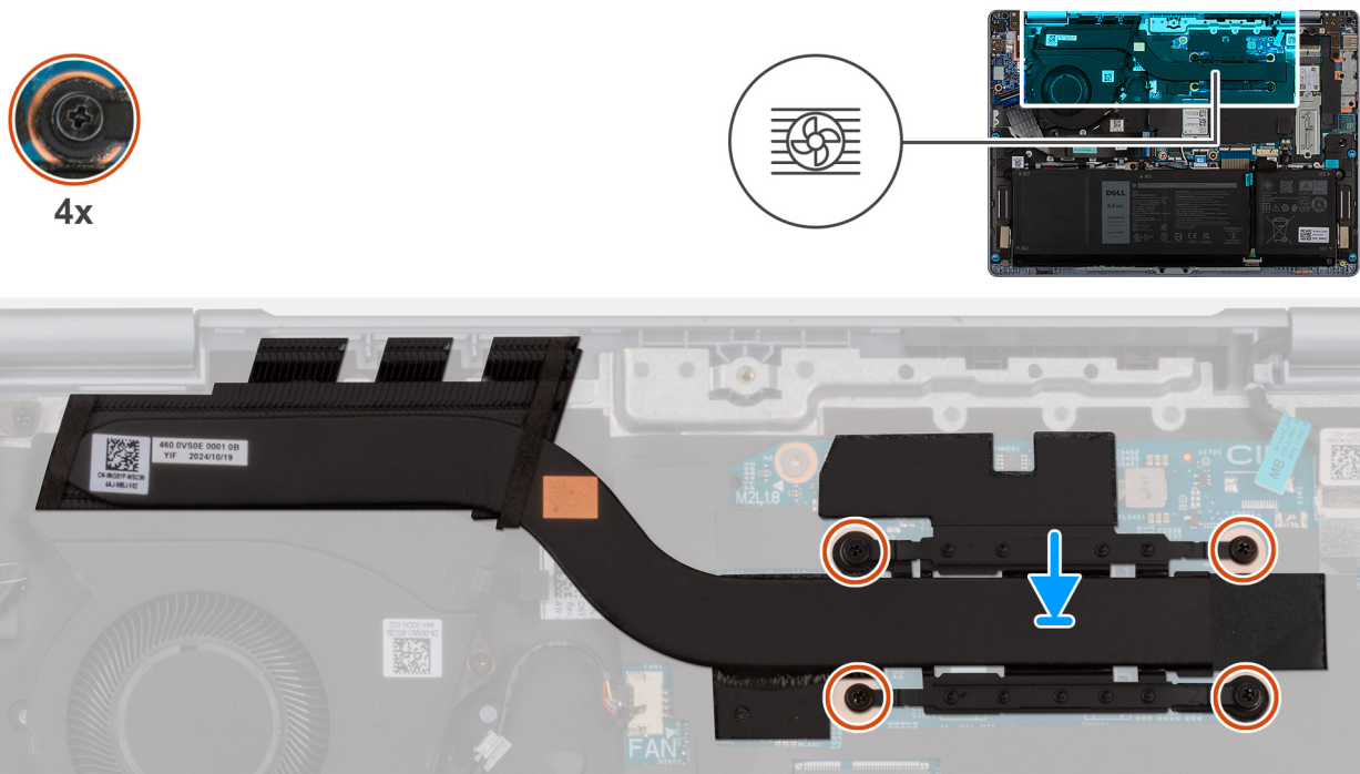
Figure 38. Installing the heat sink
