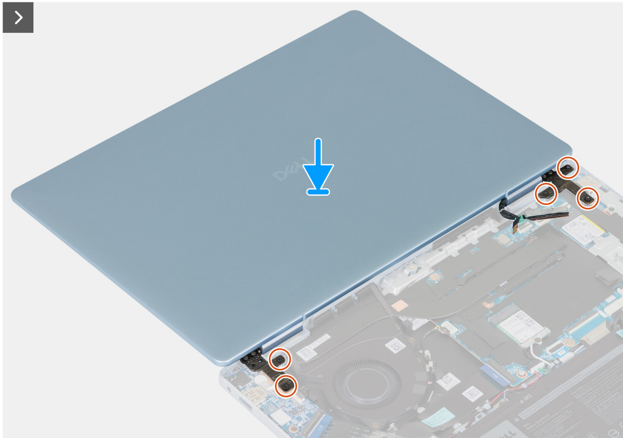
Figure 29. Installing the display assembly 1
