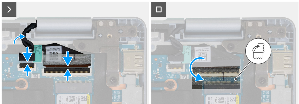
Figure 30. Installing the display assembly 2
