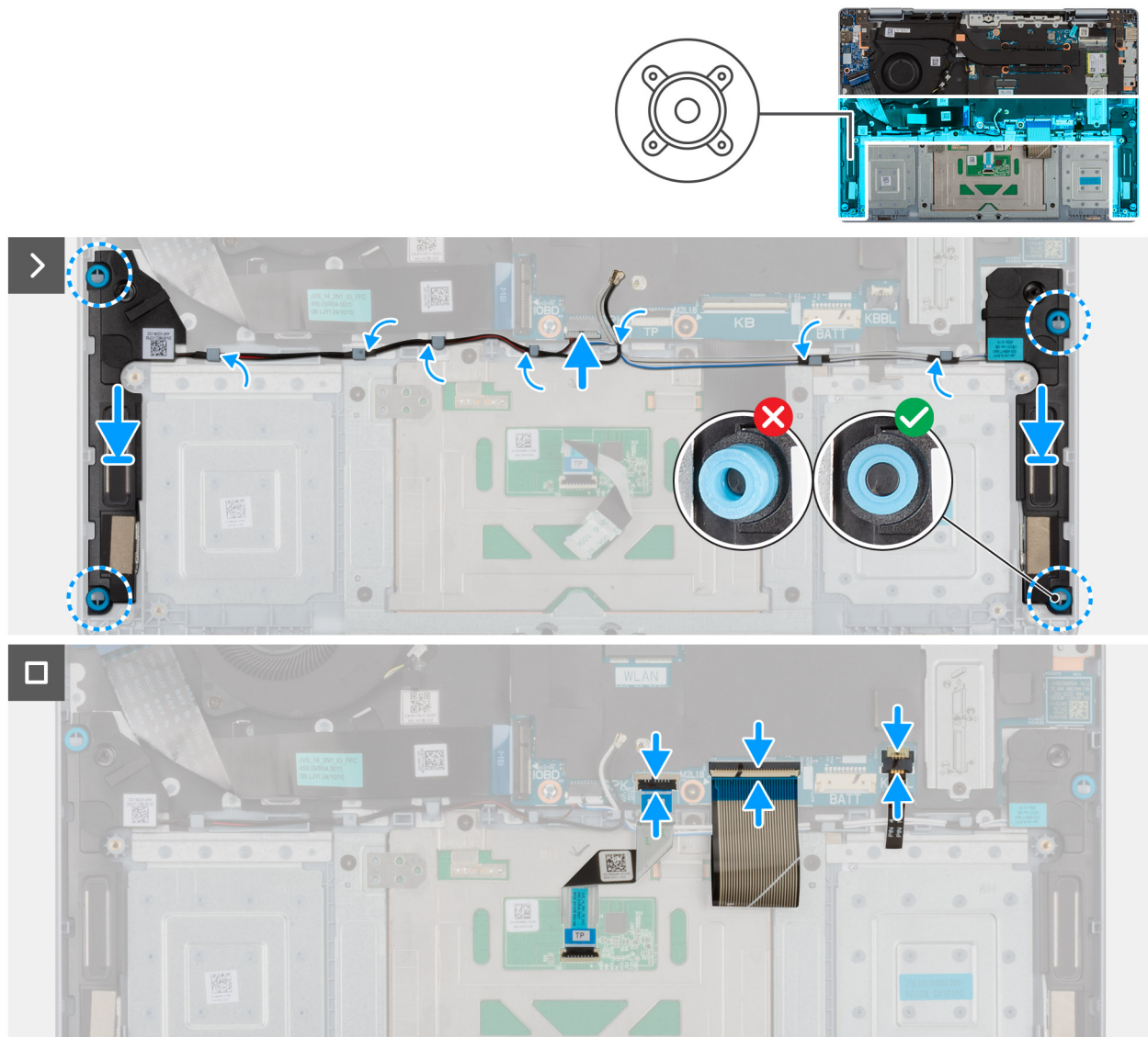
Figure 36. Installing the speaker assembly
