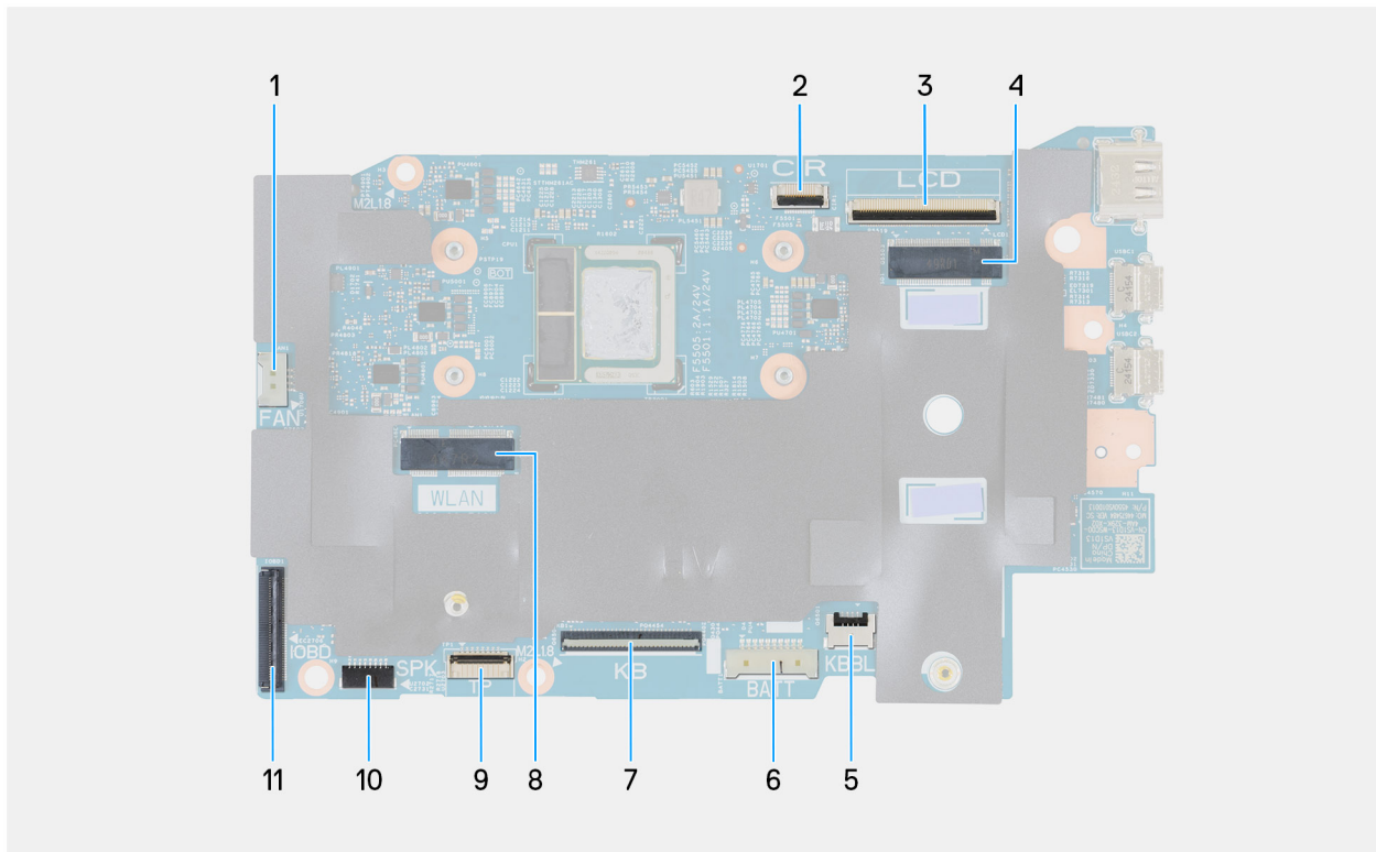
Figure 39. System board callouts
