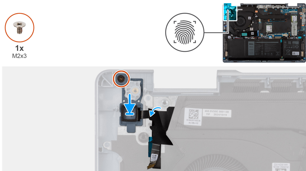
Figure 52. Installing the power button with fingerprint reader
