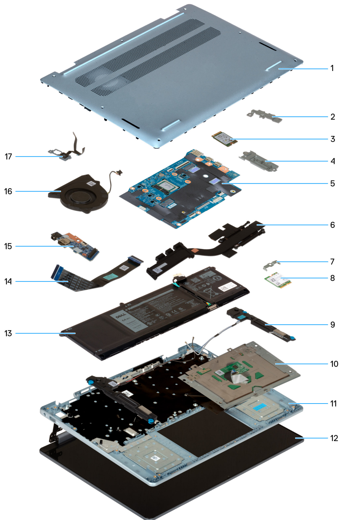
Figure 9. Image: Major components of Dell 14 Plus DB14250
