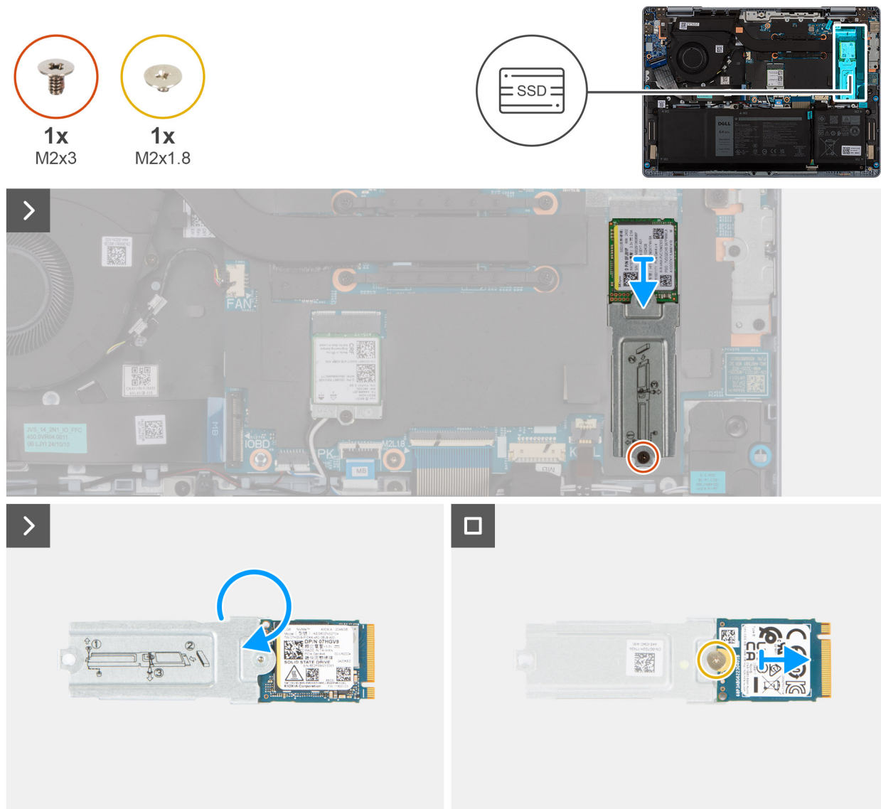
Figure 20. Removing the M.2 2230 solid state drive
