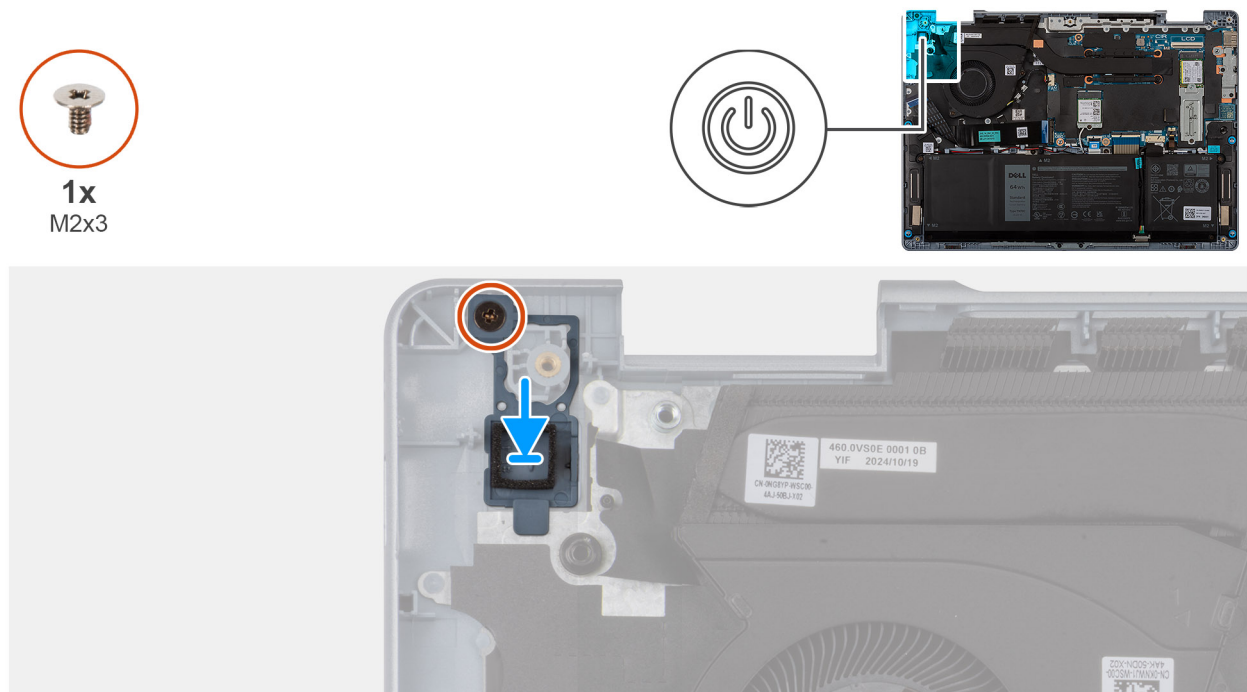
Figure 50. Installing the power button
