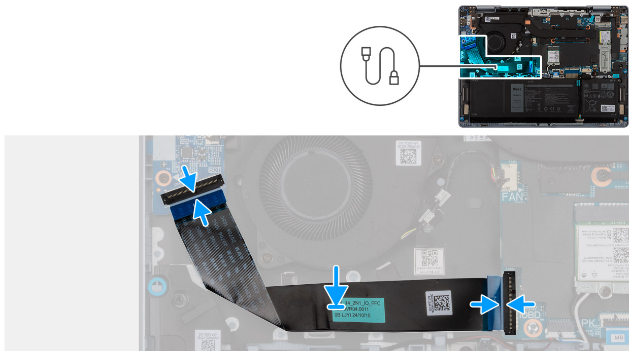
Figure 32. Installing the I/O-board cable
