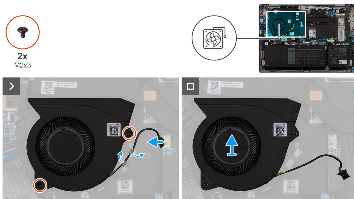
Figure 22. Removing the fan
