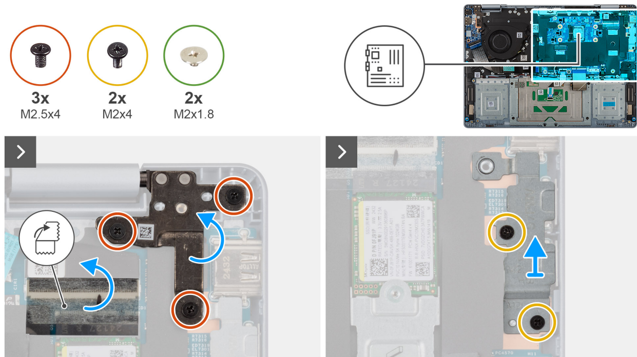
Figure 40. Removing the system board
