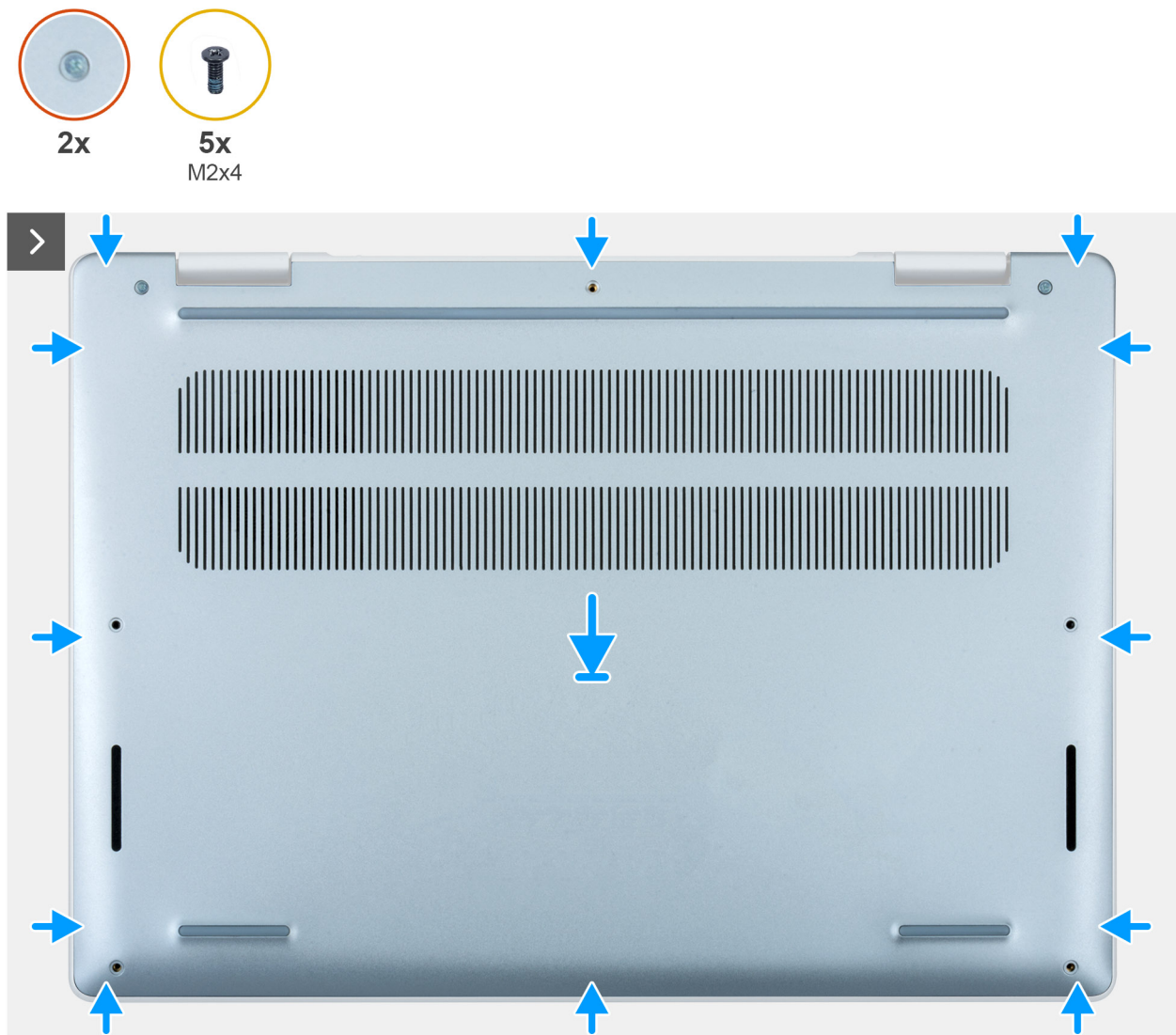
Figure 14. Installing the base cover
