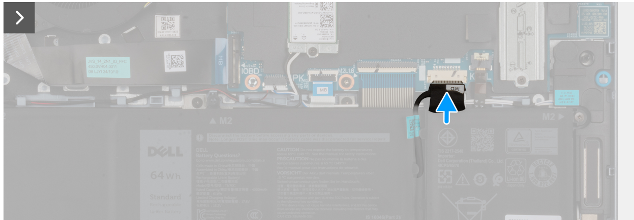
Figure 13. Connecting the battery cable
