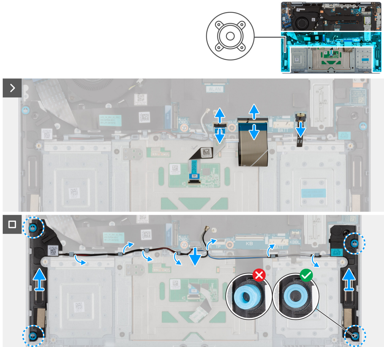
Figure 35. Removing the speaker assembly
