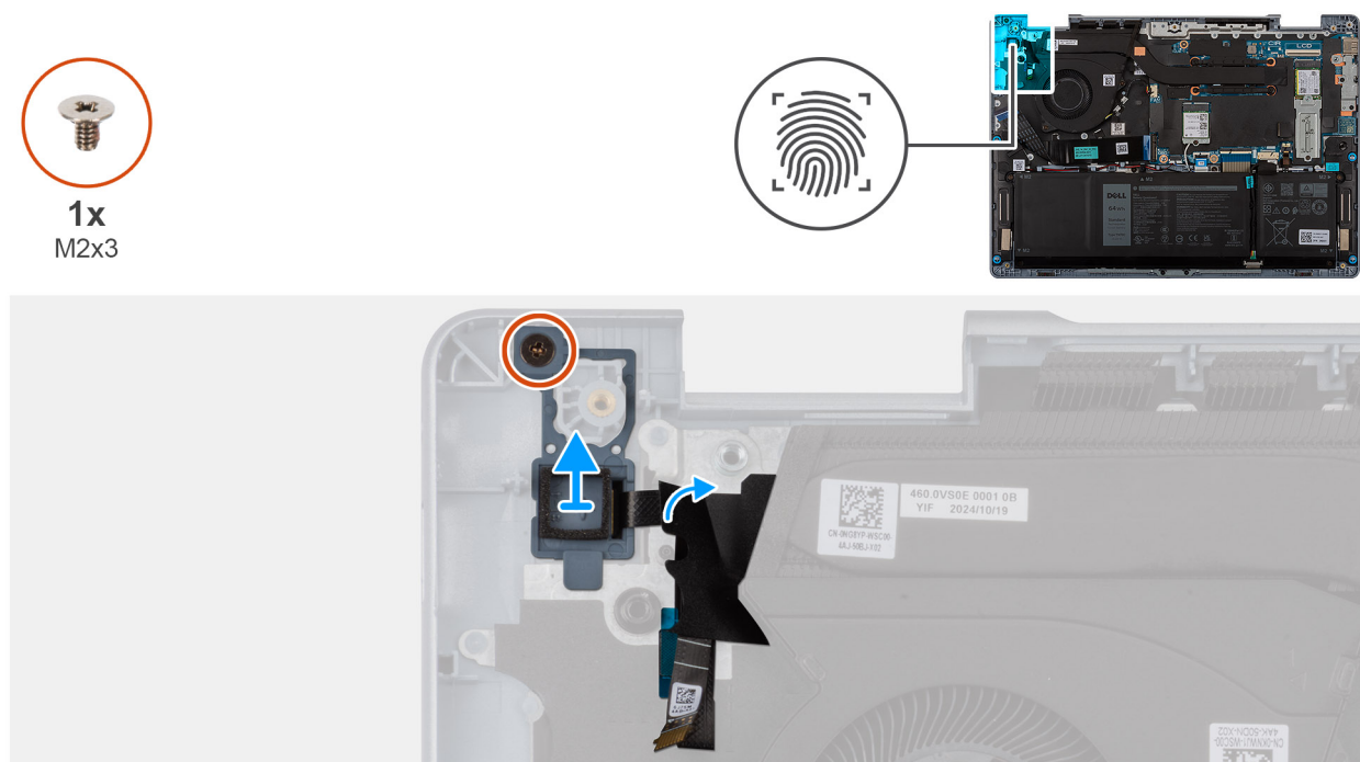
Figure 51. Removing the power button with fingerprint reader
