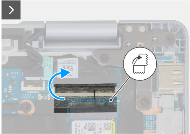
Figure 26. Removing the display assembly 1
