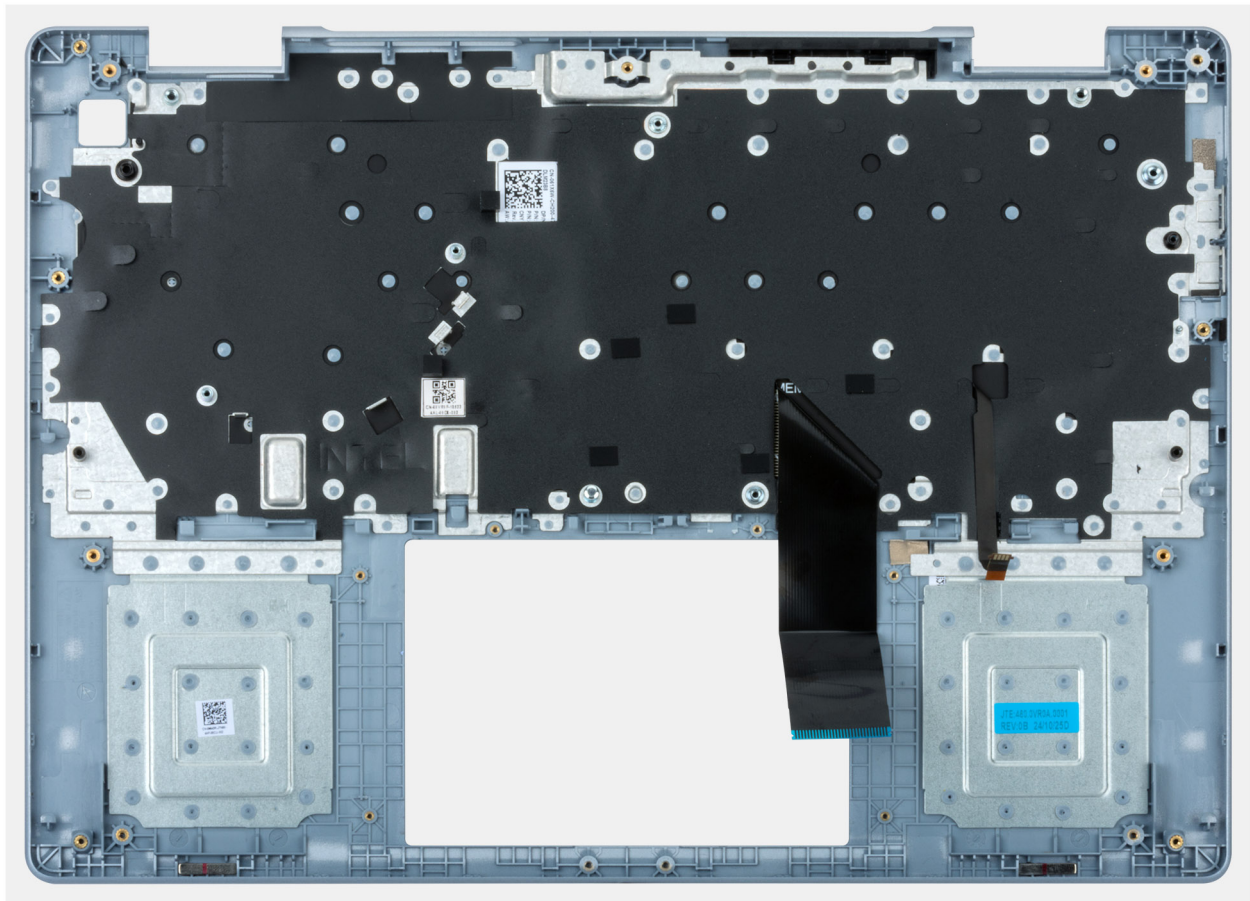
Figure 56. Palm-rest and keyboard assembly
