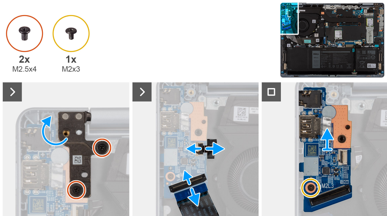
Figure 30. Removing the I/O-board
