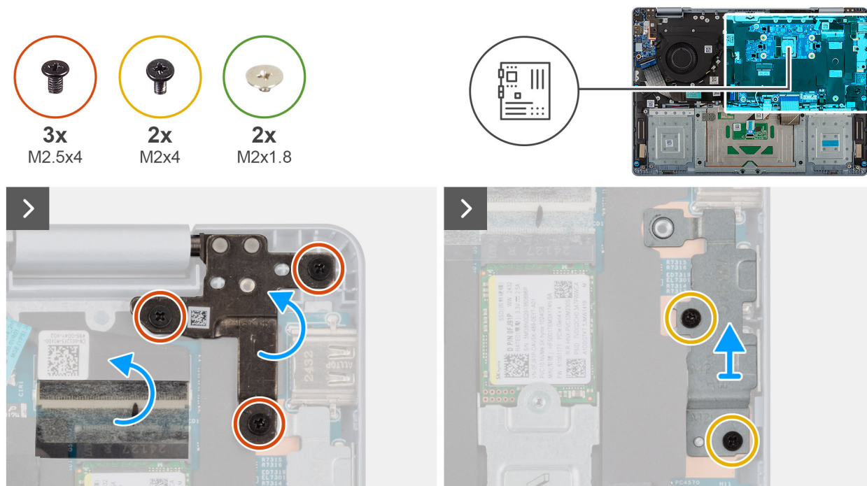
Figure 49. Removing the USB Type-C bracket and screws
