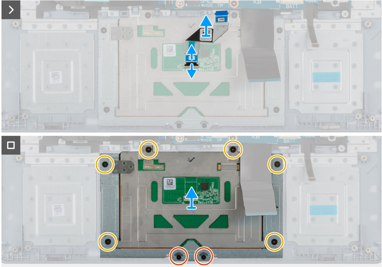
Figure 36. Removing the touchpad
