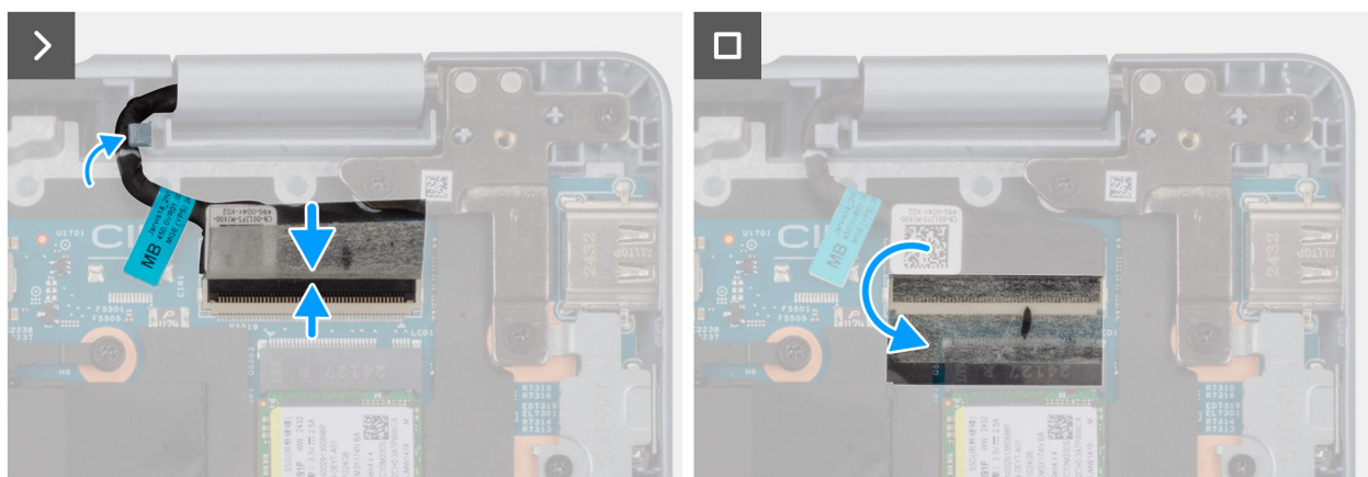
Figure 45. Connecting the display cable
