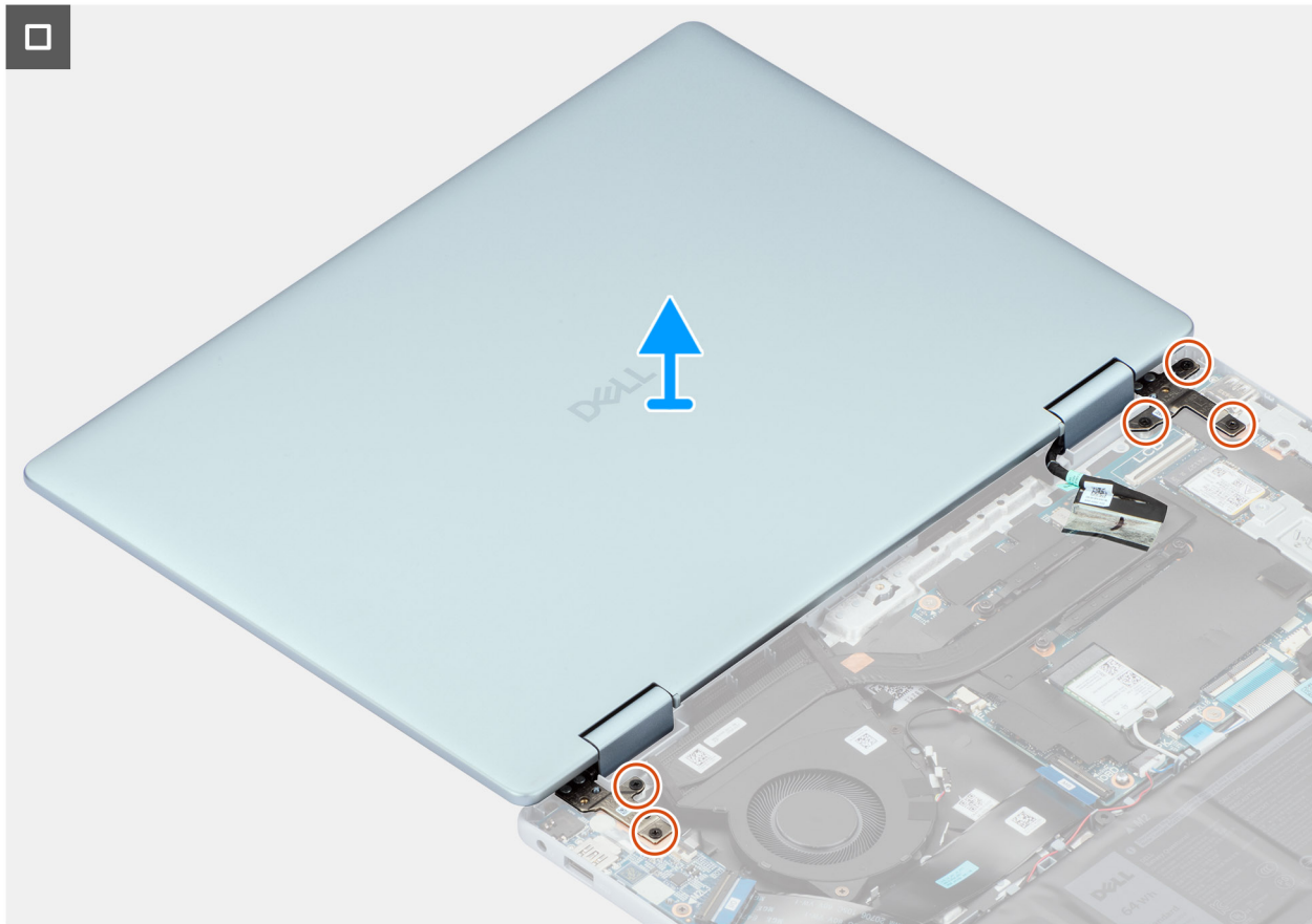
Figure 41. Removing the display assembly
