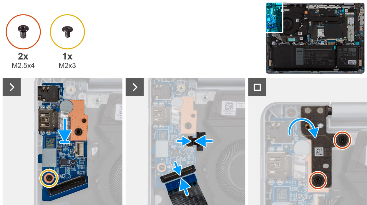
Figure 31. Installing the I/O-board
