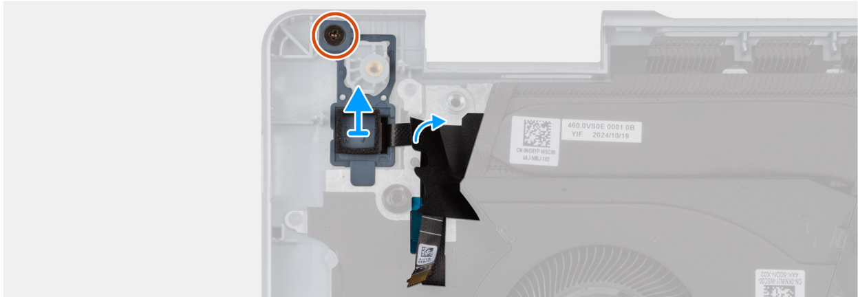
Figure 46. Removing the power button with fingerprint reader
