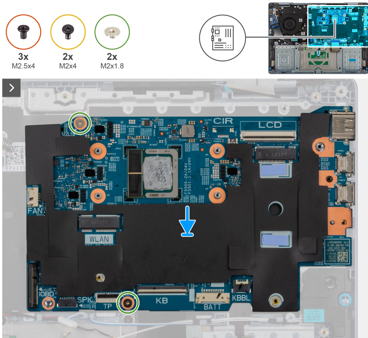
Figure 55. Installing the system board
