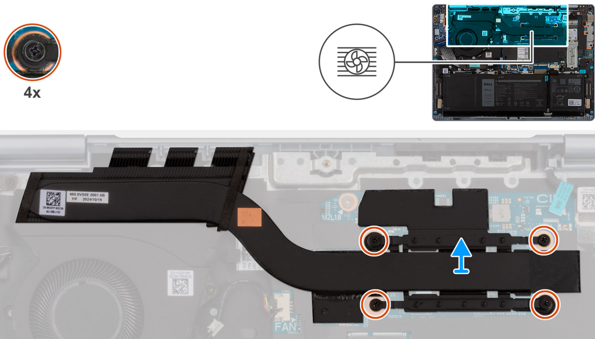
Figure 28. Removing the heat sink
