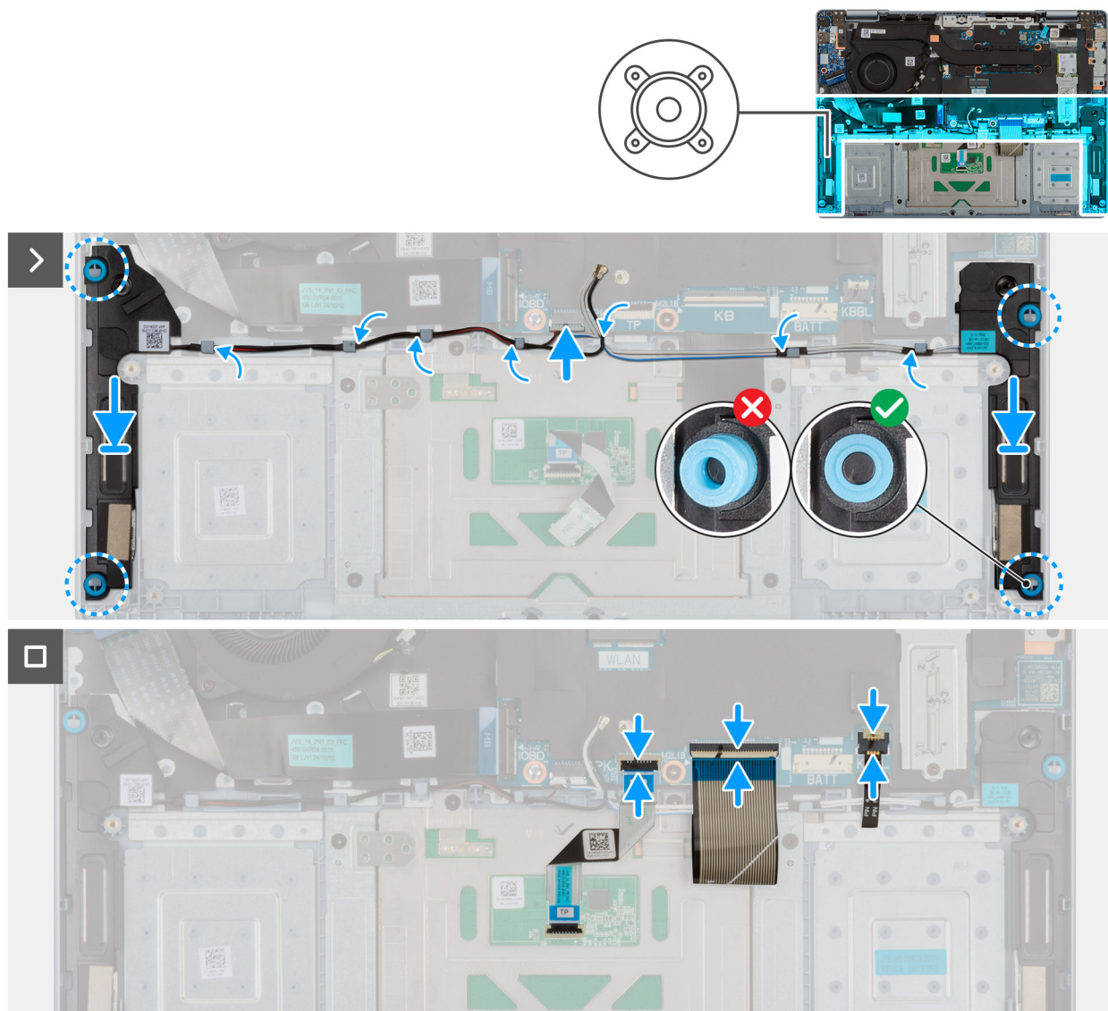
Figure 39. Installing the speakers
