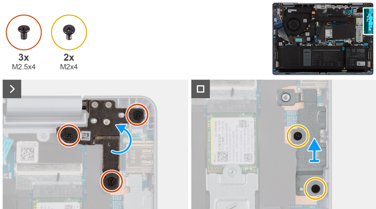
Figure 34. Removing the USB Type-C bracket
