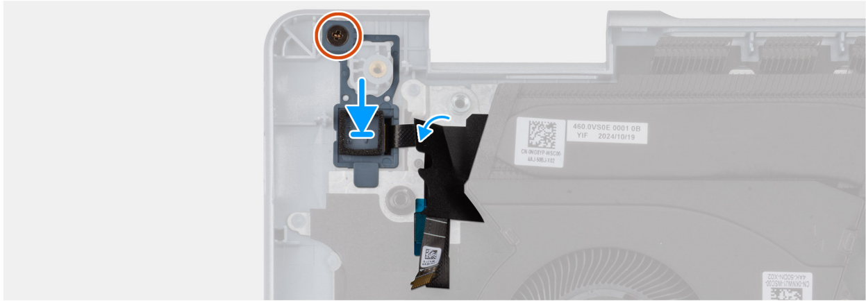
Figure 47. Installing the power button with fingerprint reader
