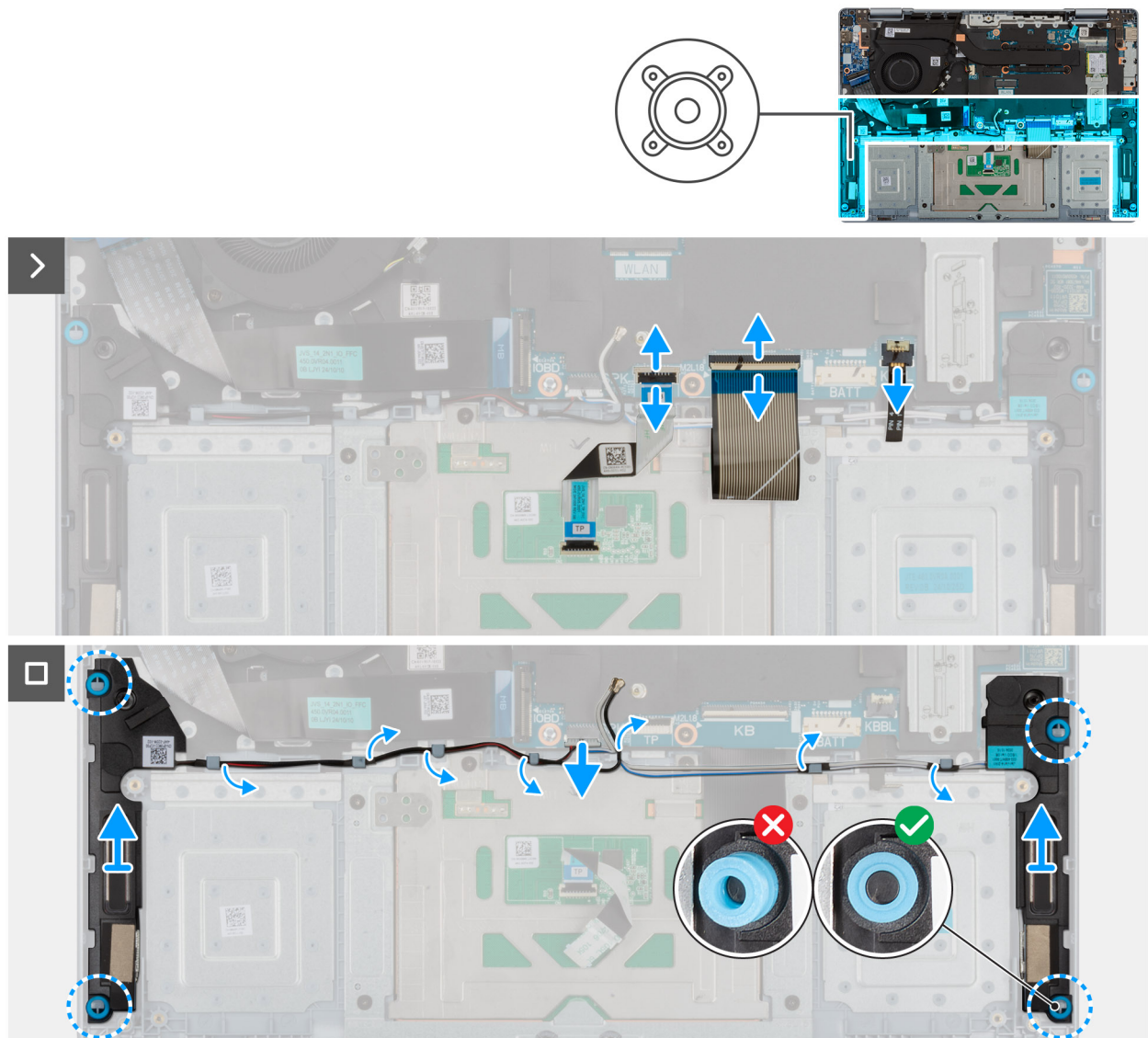
Figure 38. Removing the speakers
