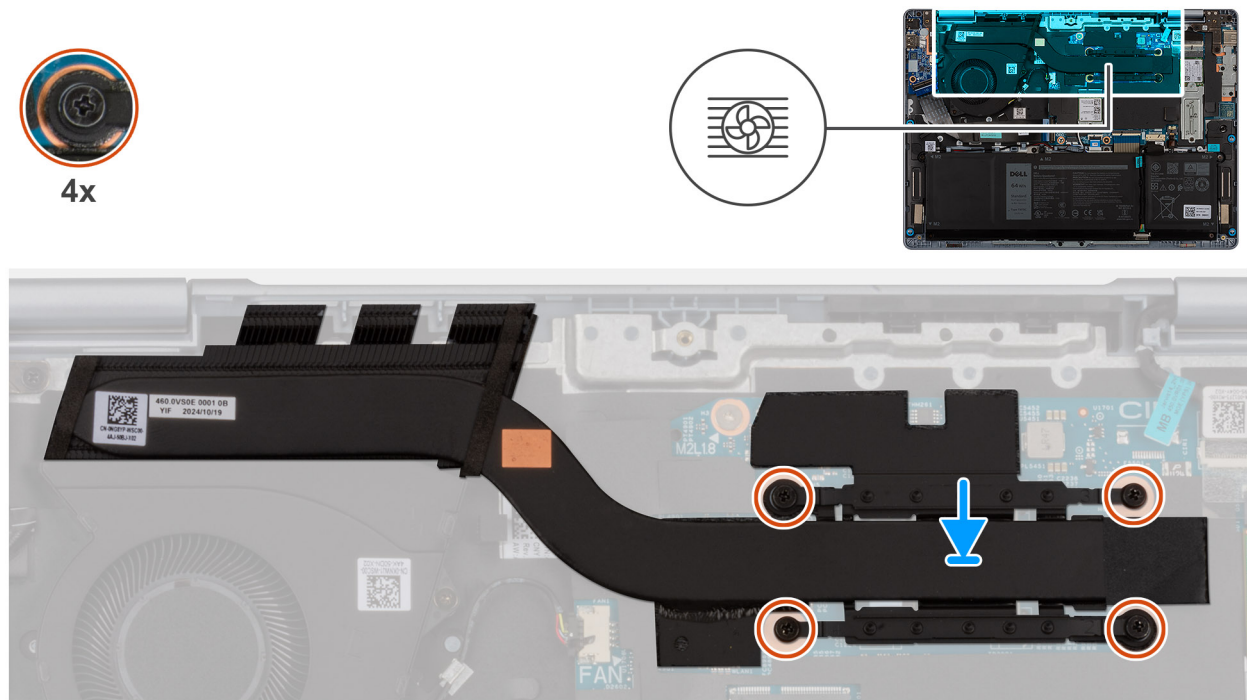
Figure 29. Installing the heat sink
