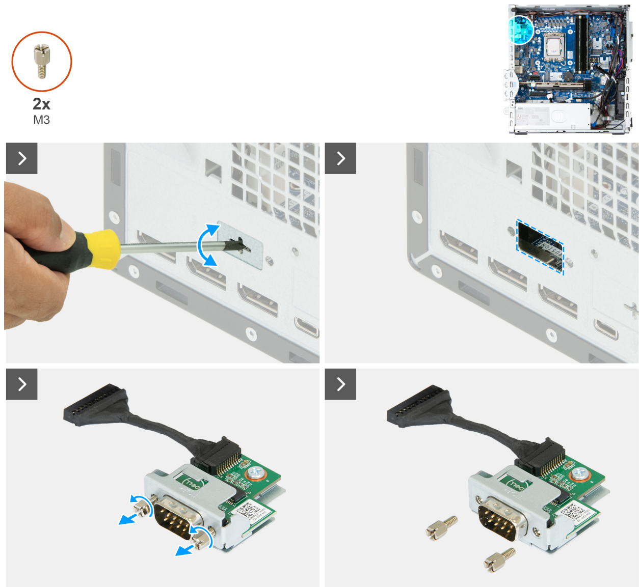
Figure 64. Installing the serial-port module
