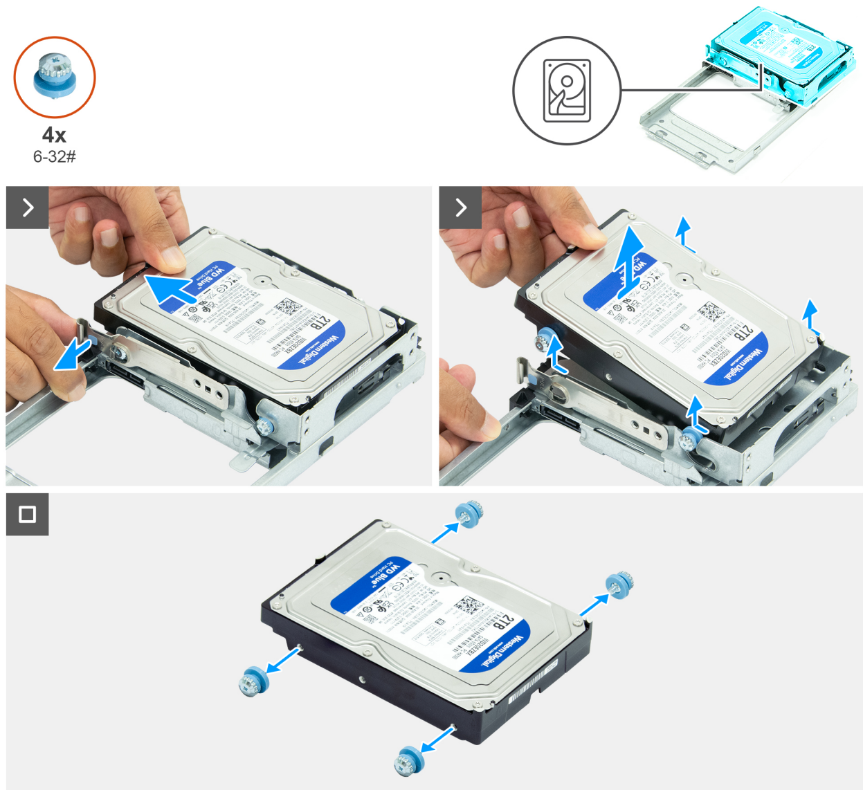
Figure 53. Removing the hard drive
