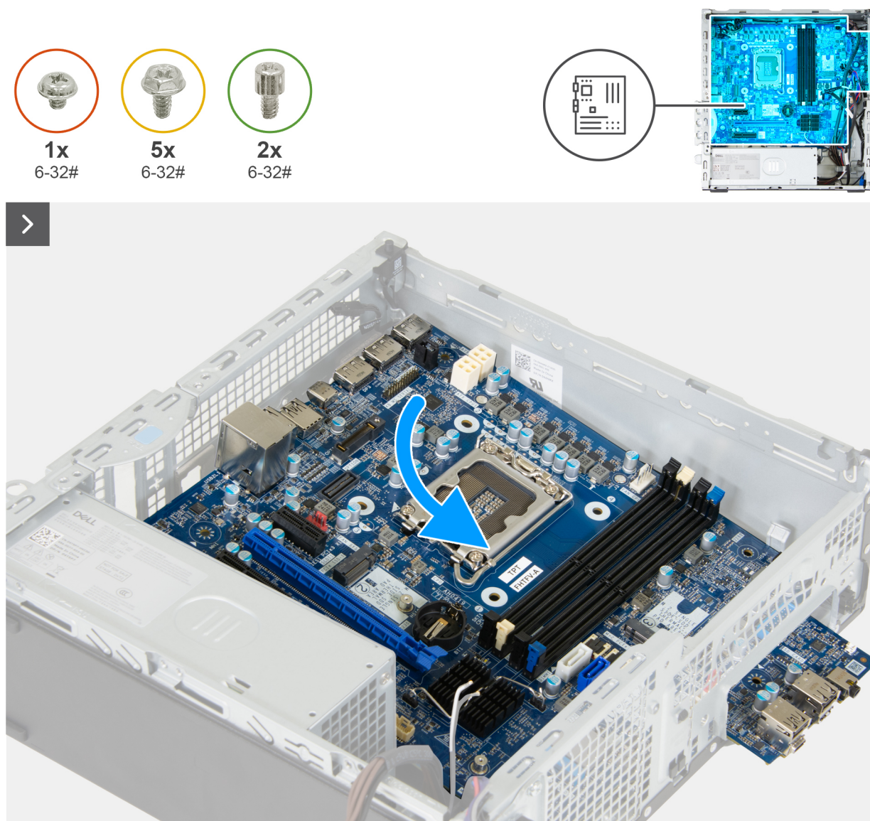
Figure 92. Installing the system board
