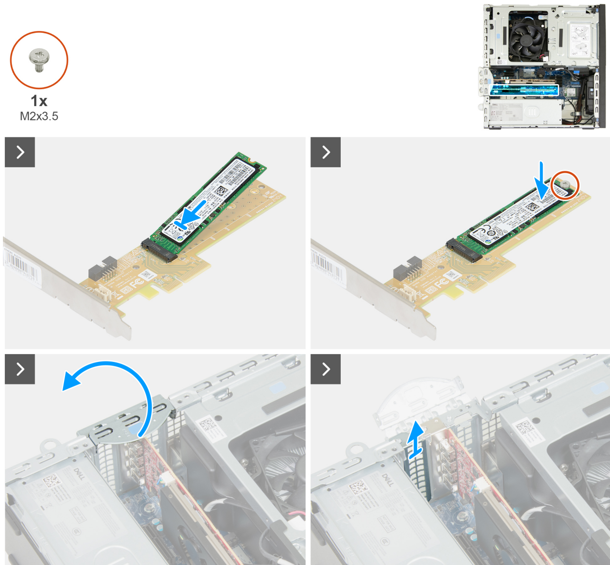
Figure 39. Installing the solid state drive expansion card
