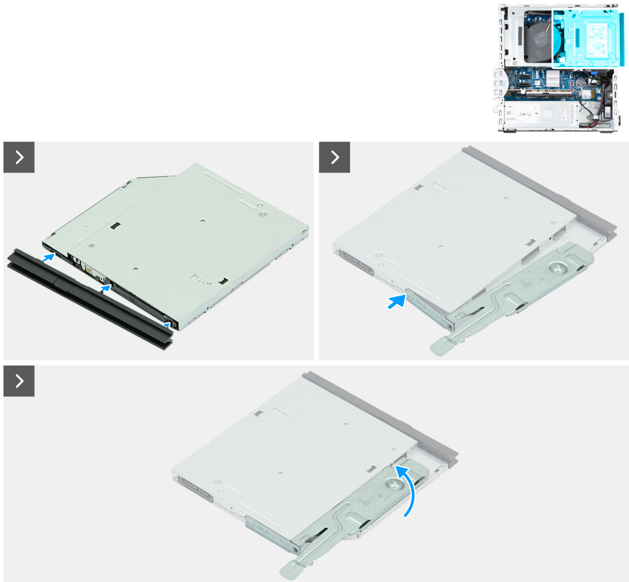
Figure 47. Installing the optical drive
