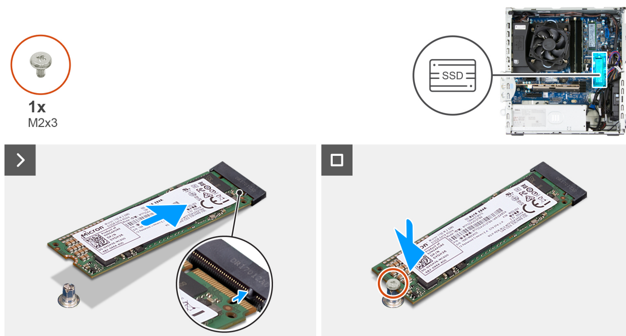
Figure 25. Installing the M.2 2280 solid state drive in slot 0
